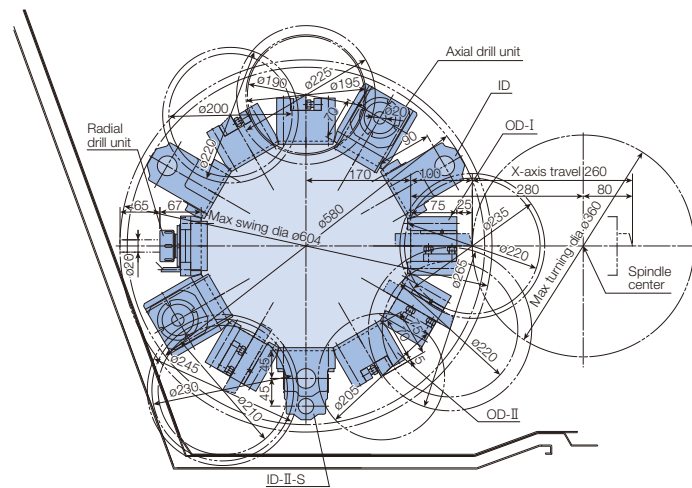
LB2000 EX III (MYW)
