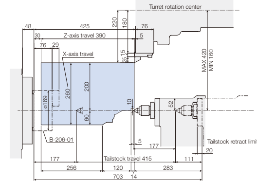
LB2000 EX III (M) C x 300 OD-I
