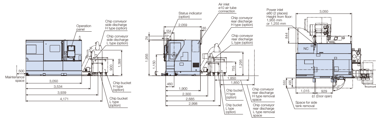
LB4000 EX III (L/M) × 1500
