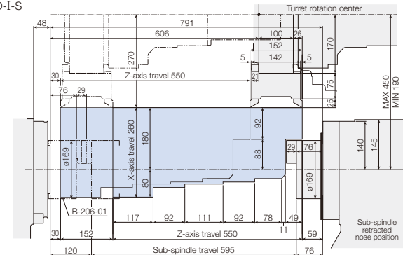
LB2000 EX III (MYW) W x 450 OD-I-S
