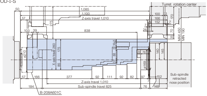
LB3000 EX III (MYW) W × 800 OD-I-S
