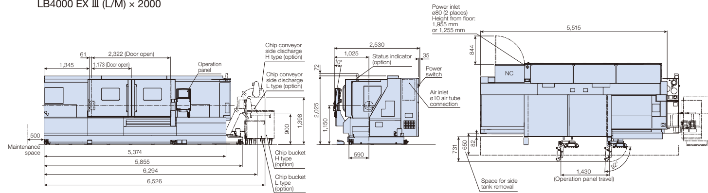
LB4000 EX III (L/M) × 2000
