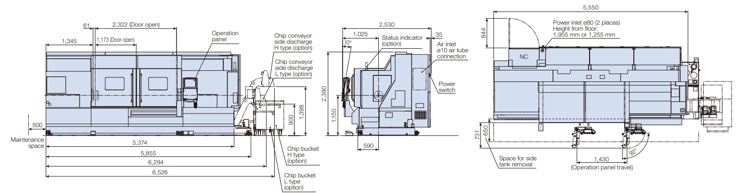
LB4000 EX III (MW) × 720
