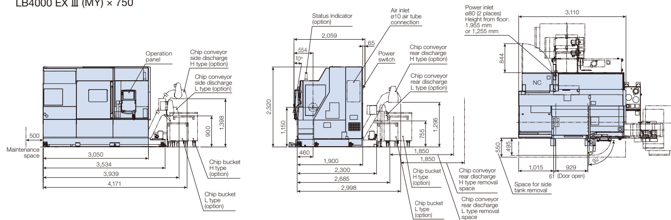
LB4000 EX III (MY) × 750
