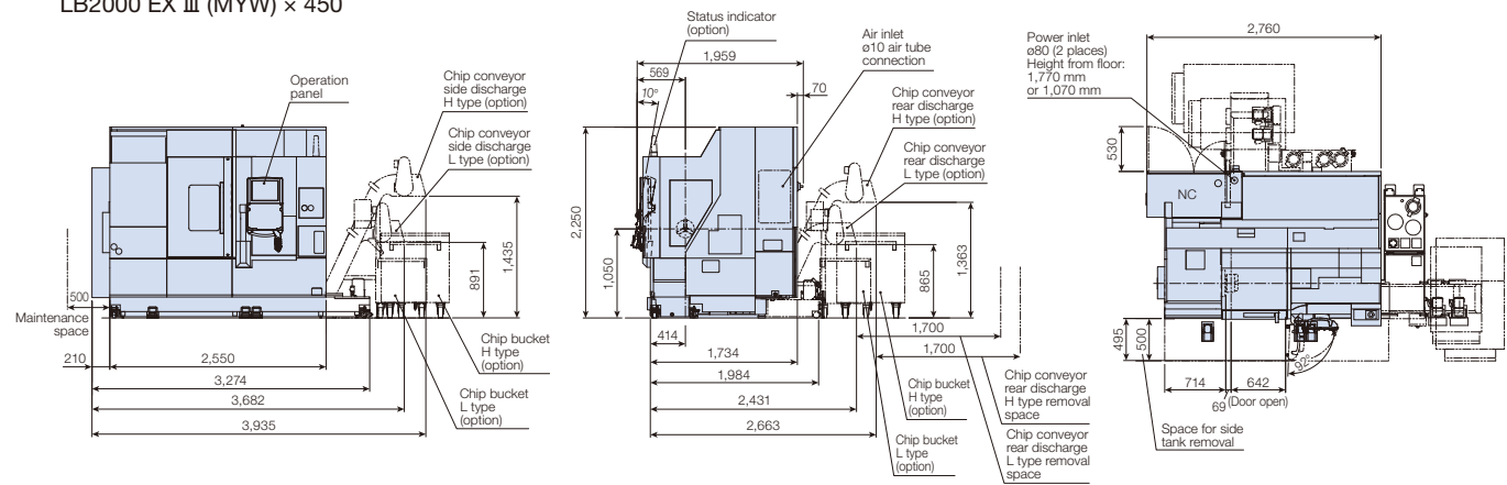
LB2000 EX III (MYW) × 450
