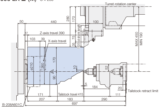
LB3000 EX III (M) C × 250 OD-I
