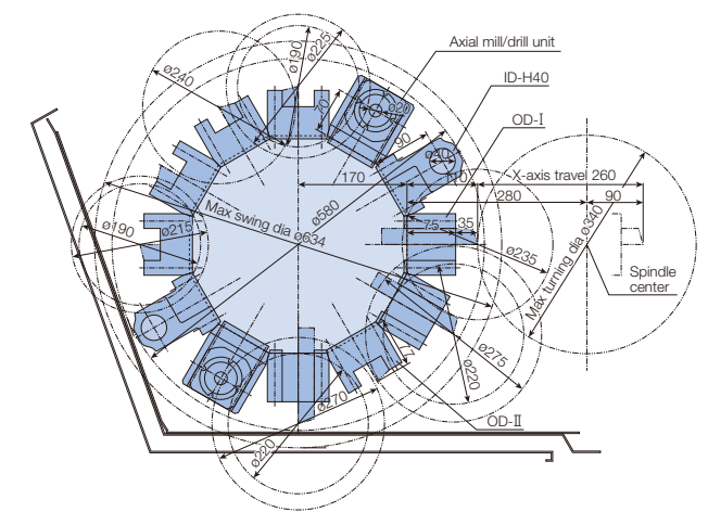
LB3000 EX III (M)
