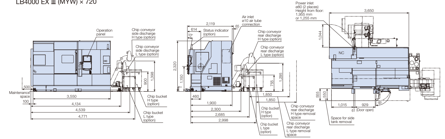
LB4000 EX III (MYW) × 720
